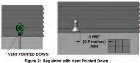
Figure 2: Regulator with Vent Pointed Down
