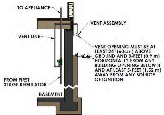
Figure 4: Basement Installation
