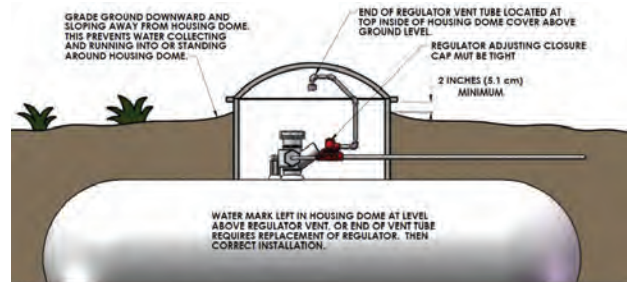
Figure 5: Underground Installation
