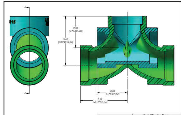
MEP995SBW-16 vs. standard tee
