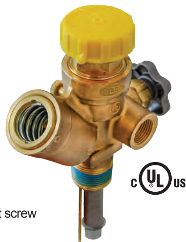
MES-PVE2035AT Multi-Service Valve
